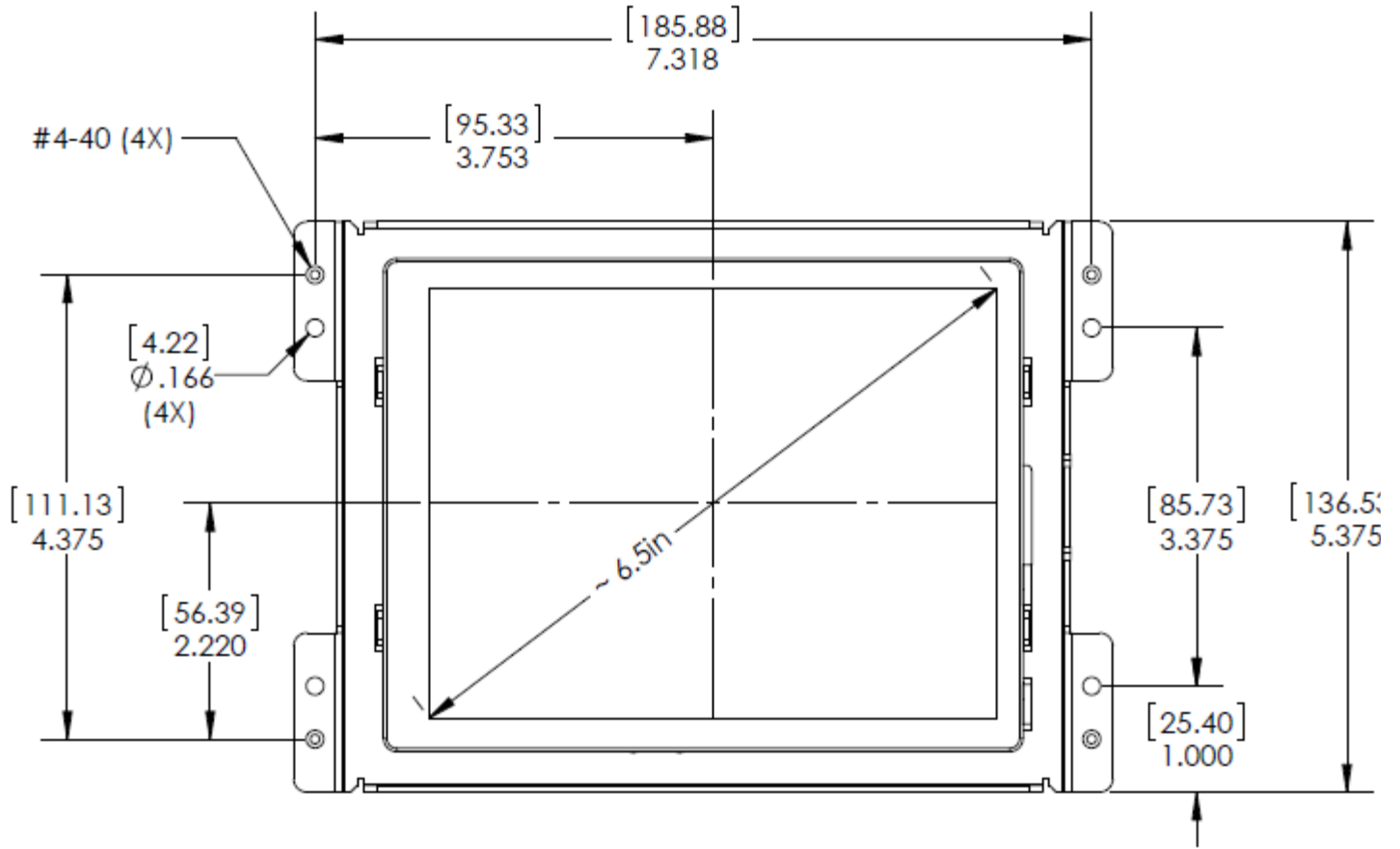
Front View (Panel)
