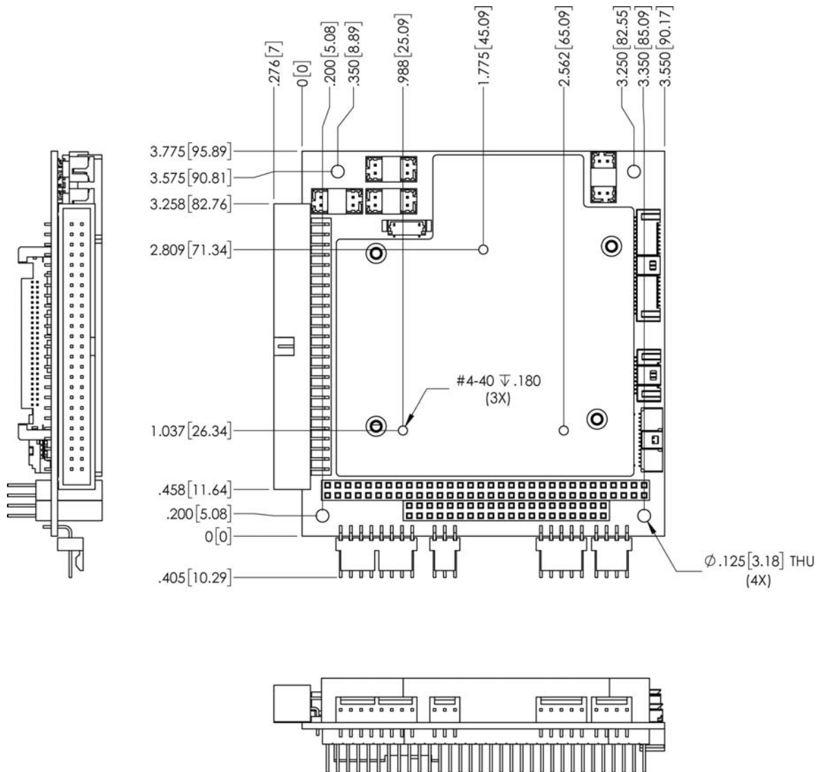
PCM-C418 Drawing, Top and Side Views
