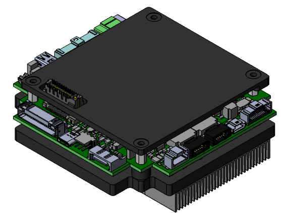
ISOMETRIC VIEW SCALE 1:2
