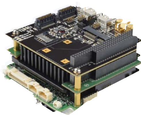
Two-board Stack with RISER Extender Cards
